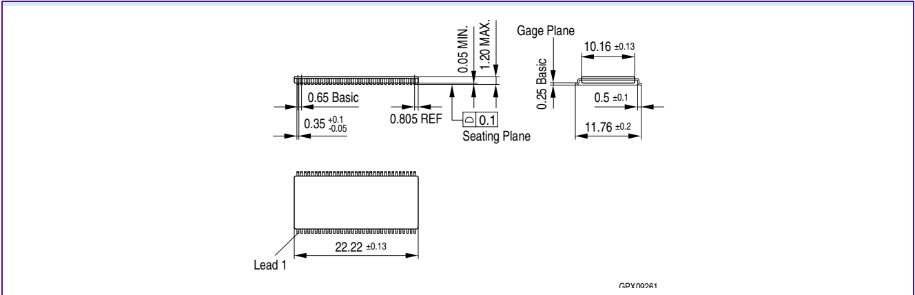
FIGURE 5 Package Outline of P-TSOPII-66-1 (non-green/green)
